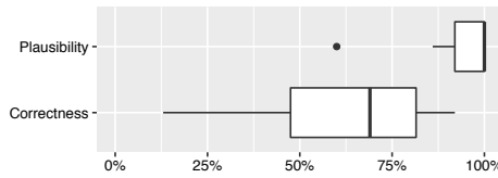
Figure 7: Boxplots showing the proportional patch correctness and plausibility. For instance, if the proportional patch correctness for an error is 50%, then half of the patches submitted for this error are correct. The boxplot shows the proportional plausibility and correctness over all 27 errors.
