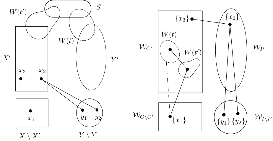
Figure 3: Left hand side figure shows partition (S, X, Y) of G where as right hand side figure shows witness sets in G and G' . We need to modify witness sets in \mathcal{W}_I which are adjacent with each other (e.g. \{y_1\} and \{x_2\} ) and witness sets in \mathcal{W}_C which are not adjacent with each other (e.g. W(t) and \{x_1\} ). Please refer to Lemma 4.3.
