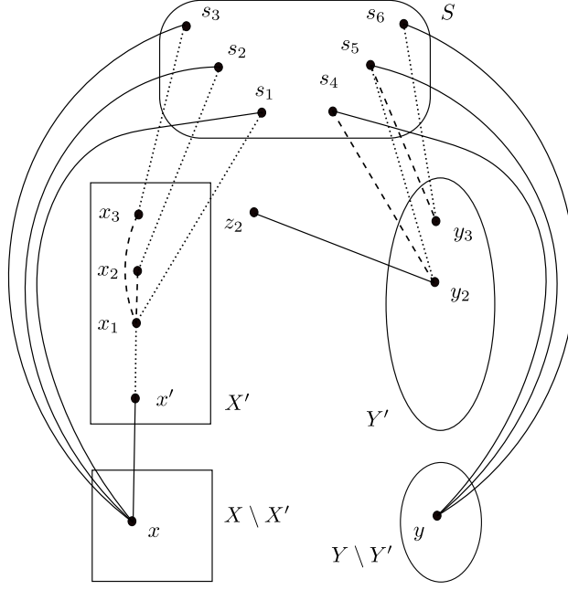
Figure 4: Straight lines (e.g. xx' ) represent edges in original solution F . Dotted lines (e.g. x_1x' ) represents an edges replaced in F . Dashed lines (e.g. x_1x_2 ) represents extra edges added to F . Please refer to Conditions 2 and 3 in Lemma 4.4. Vertex z_2 can be in X or S .
