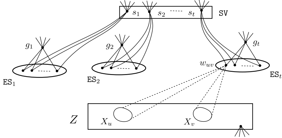
Figure 5: Sets with rectangular boundary represent cliques whereas sets with elliptical boundary represent independent sets. A vertex w_{uv} , corresponding to an edge uv , is adjacent to all vertices in Z except the ones in X_u \cup X_v . Dashed lines shows non-adjacency between the vertex and sets. Please refer to reduction from MULTICOLORED DENSEST- k -SUBGRAPH WITH PERFECT COMPLETENESS to SPLIT CONTRACTION for details.
