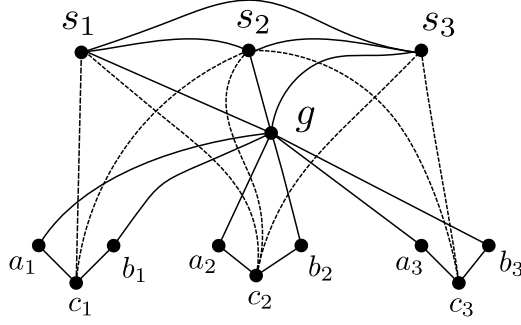
Figure 6: Reduction from an instance ((U, \mathcal{S}), k) of SET COVER to an instance (G, k) of CHORDAL CONTRACTION. Here U = \{u_1, u_2, u_3\} ; \mathcal{S} = \{S_1, S_2, S_3\} where S_1 = \{u_1, u_2\} , S_2 = \{u_1, u_2, u_3\} , and S_3 = \{u_2, u_3\} . Straight lines (eg. a_1g ) are part of gadget construction whereas dashed lines (eg. c_1s_1 ) are added because of containment relationship between elements and sets. Please refer to the Reduction Algorithm in the proof of Lemma 6.1.
