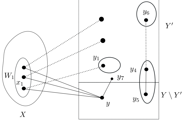
Figure 2: Straight lines (e.g. y_4y_5 ) represent edges in original solution F . Dotted lines (e.g. y_4y_6 ) represents edges which are replaced for some edges in F . Please refer to the proof of Lemma 3.4.
