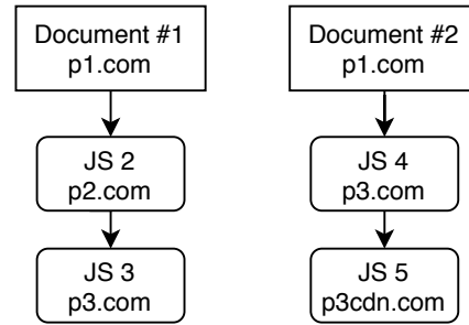
Fig. 1. Example inclusion trees
